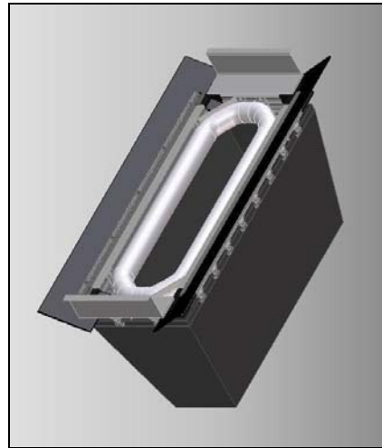
StormSack, Type H Flange (Assembled)
