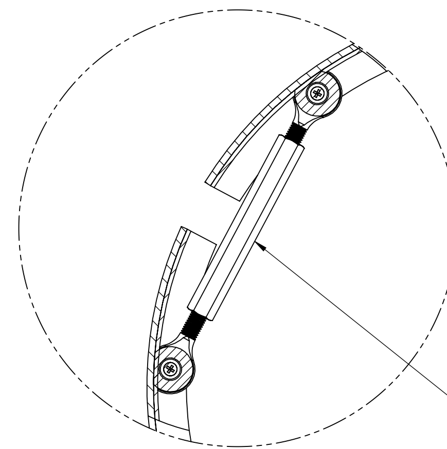
CUTAWAY DETAIL
